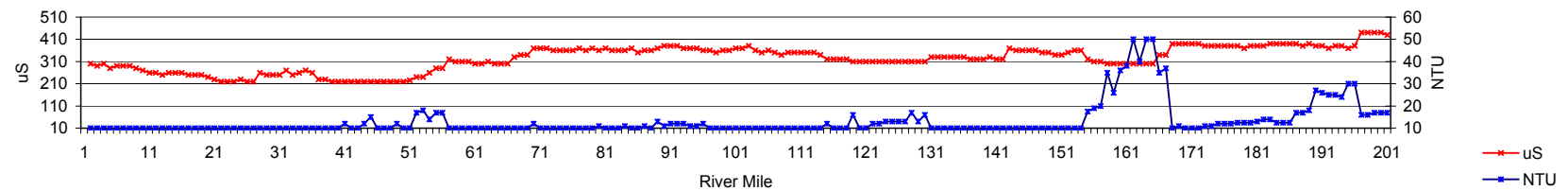
Meramec River Mile Conductivity (uS) & Turbidity (NTU) 2008
